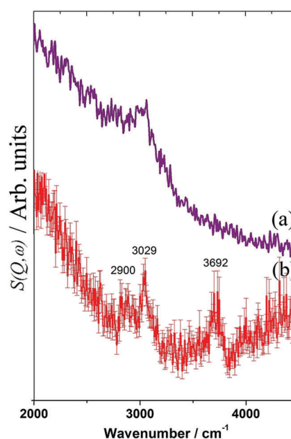
Fig. 17 INS spectra of a Ni(26%)/Al 2 O 3 catalyst after (a) dry reforming and (b) steam reforming of methane at 898 K for six hours.
