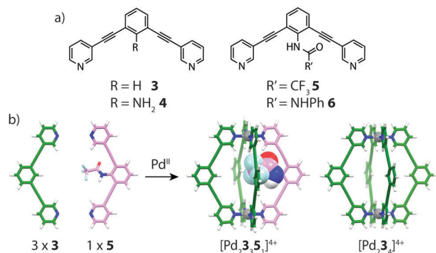
Fig. 5 (a) Endohedrally functionalized ligands 3–6 bearing varying degrees of steric bulk; (b) integrative self-sorting of ligands 3 and 5 to give a 3 : 1 mixture of [Pd_2 3_3 1]^{4+} and [Pd_2 3_4 1]^{4+} . The NHCOCF 3 endohedral substituent in the heteroleptic assembly is shown as a space-filling representation.
