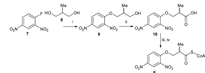
Scheme 2 Synthesis of substrate 6. Reagents & conditions: (i) Na metal, 83%; (ii) CrO 3 , conc. H 2 SO 4 , acetone, 67%; (iii) carbonyldiimidazole, CH 2 Cl 2 ; (iv) CoA-SH (Li + ), 0.1 M NaHCO 3 aq./THF (1:1).
