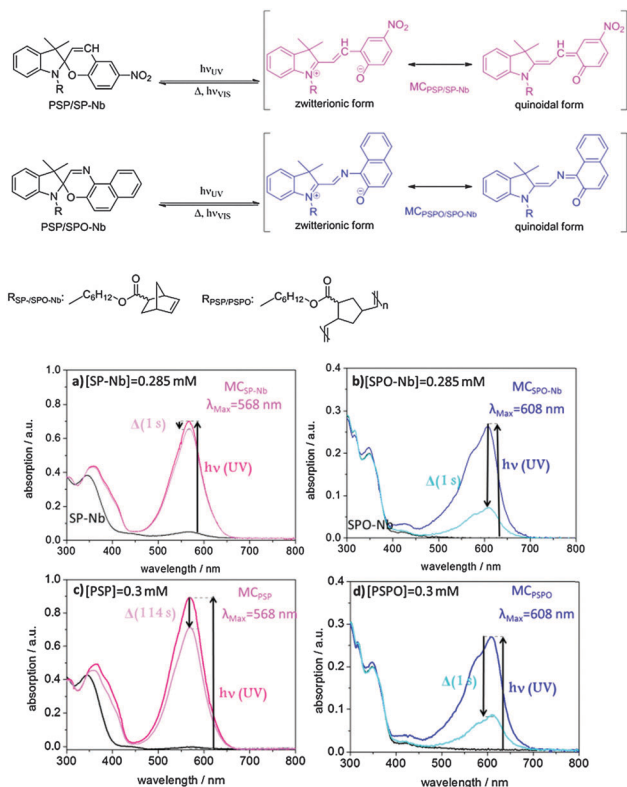
Fig. 2 Schematic description of the photochromic mechanism in spirooxazine and spiropyran containing species and UV/VIS-spectroscopic measurements in DMF of (a) SP-Nb, (b) SPO-Nb, (c) PSP and (d) PSPO in DMF (dry) under a nitrogen atmosphere. The absorption spectra before irradiation are shown in black. The absorption spectra directly after irradiation and in darkness at room temperature are shown in light blue and pink for SPO and SP, respectively.
