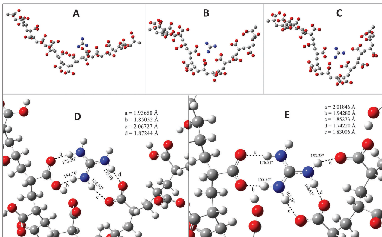
Fig. 6 Details of DFT studies have been depicted. In (A), oxygen atoms of the \text{COOH} group form hydrogen bonds with N-H of GD molecules. Panels B and C show the gradual increase in interaction among GD and PAA inside a single PAA chain with the increase in the number of free -\text{COO}^- and this enhanced interaction results in coiling of the PAA forming PAA-GD clusters. Panels D and E are the close-up views of panels B and C respectively where the hydrogen bonded distances are shown. It is clearly seen that most of the hydrogen bonds are getting shortened and formation of more hydrogen bonds is also seen with enhanced interaction between PAA and GD.
