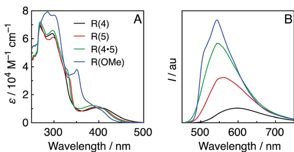
Fig. 1 UV-vis (A) and emission (B) spectra of the Re-rings in DMF under Ar. The emission spectra were corrected to the absorbed photons at \lambda_{ex} = 400 nm.
