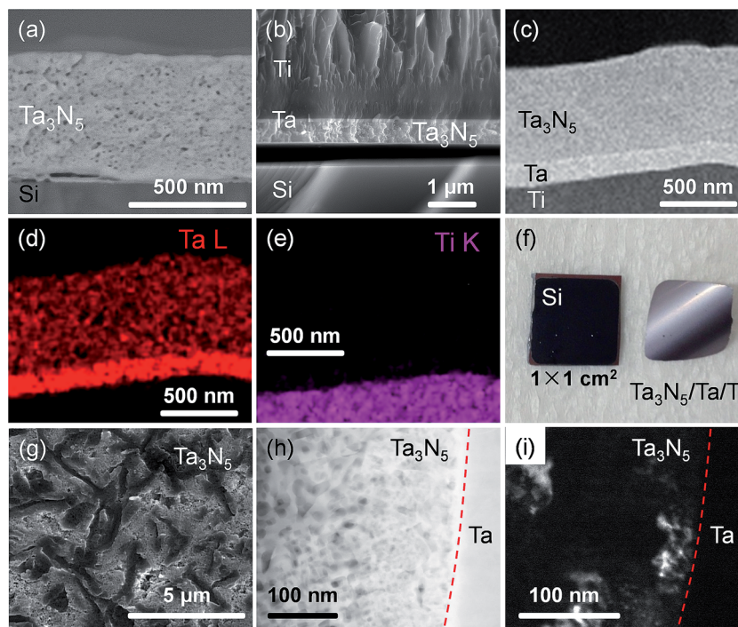
Fig. 3 Cross-sectional SEM images of (a) Ta 3 N 5 /Si and (b) Ti/Ta/Ta 3 N 5 /Si, (c) cross-sectional STEM image of transferred Ta 3 N 5 /Ta/Ti, EDS maps for (d) Ta and (e) Ti taken from the STEM image in panel (c), (f) digital photographs of a Ta 3 N 5 /Ta/Ti sample transferred from a Si substrate, (g) top-view SEM image of a Ta 3 N 5 /Ta/Ti sample, and dark-field (h) STEM and (i) zone-axis TEM images of a Ta 3 N 5 /Ta/Ti sample near the Ta 3 N 5 /Ta interface.
