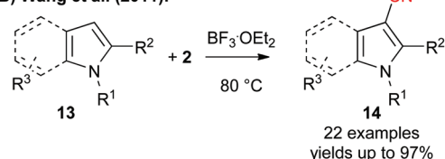
Scheme 2 NCTS (2) in the direct synthesis of aryl-carbonitriles.
