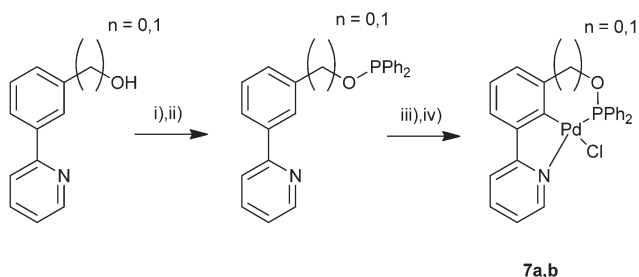
Scheme 8 Synthesis of PCN pincer palladacycles. (i) \text{NEt}_3 , \text{DMAP} , \text{Et}_2\text{O} 0^\circ\text{C} . (ii) \text{ClPPh}_2 , rt. (iii) \text{Pd}(\text{OAc})_2 , \text{AcOH} . (iv) \text{NaCl} , \text{H}_2\text{O}/\text{MeCN} . 7a n = 1 , 7b n = 0 .
