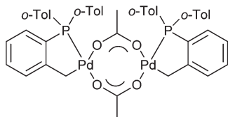
Fig. 1 Herrmann–Beller palladacycle.
