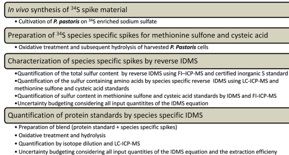
Fig. 1 Experimental workflow of the introduced species specific IDMS method addressing protein quantification by the sulfur containing amino acids.
