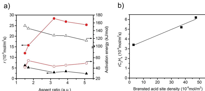
Fig. 6 (a) Specific reaction rates measured at T = 310\text{ }^{\circ}\text{C} and normalized to surface area, and apparent activation energy as a function of the aspect ratio; red solid circle: acetaldehyde formation rate; red open circle: apparent activation energy of acetaldehyde formation; black solid triangle: ethylene formation rate; black open triangle: apparent activation energy of ethylene formation; (b) rate of formation of ethylene as a function of Brønsted acid site density at the catalyst surface determined by ammonia adsorption and specific surface area measurements.
