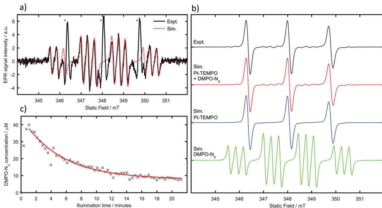
Fig. 3 (a) Overlap of experimental and simulated DMPO- N_3 adduct spectra. The experimental trace shows the subtraction of spectra recorded immediately before and after switch on of the light source. Stars indicate the location of the three main lines in the TEMPO spectrum which are not fully subtracted; (b) comparison between simulated and experimental EPR spectra of Pt-TEMPO and DMPO- N_3 ; (c) azide spin-adduct concentration as a function of illumination time (42 mW at 405 nm) determined by least-squares fitting of the sum of simulated Pt-TEMPO and DMPO- N_3 spectra to the experimental EPR traces.
