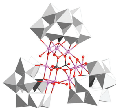
Fig. 36 Structure of the nonanuclear Co-POM [\text{Co}_9(\text{OH})_3(\text{OH})_6(\text{HPO}_4)_2(\text{PW}_9\text{O}_{34})_3]^{16-} ( 89 ). Adapted with permission from ref. 247. Copyright 2012 American Chemical Society.
