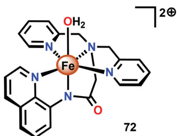
Fig. 30 Structure of the [Fe(dpaq)(OH 2 )] 2+ complex 72.
