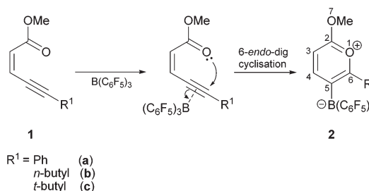
Scheme 1 Proposed mechanistic pathway of the reaction between \text{B}(\text{C}_6\text{F}_5)_3 and methyl en-ynoates.
