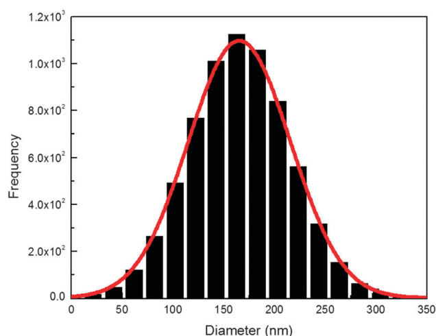
Fig. 5 Particle size distribution of ZnCoS thin films.
