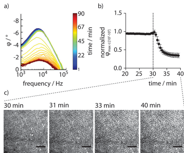
Fig. 4 Monitoring of epithelial barrier disruption by ionomycin using the transparent conductive polymer-based 2-electrode PAS sensor. (a) Partial PAS spectra of cells exposed to ionomycin after 30 min baseline recording. Spectra were achieved at 10^3 – 10^5 Hz with 30 s time resolution. The colour-coded time parameter shows decay of epithelial integrity by the decreased amplitude of the peak \varphi values. (b) Extracted, normalized \varphi peak values show the kinetics of epithelial barrier degeneration. (mean \pm SEM, n = 3 ). (c) Phase contrast microscopy performed simultaneously to PAS sensing. (20 \times , scale bar = 200 \mu m).
