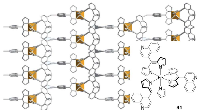
Fig. 18 Metal-organic framework comprising tris(dipyrinato)iron(III) complex 41 with 4-quinoyl groups at the meso -position. Adapted with permission from ref. 88. Copyright 2006 American Chemical Society.
