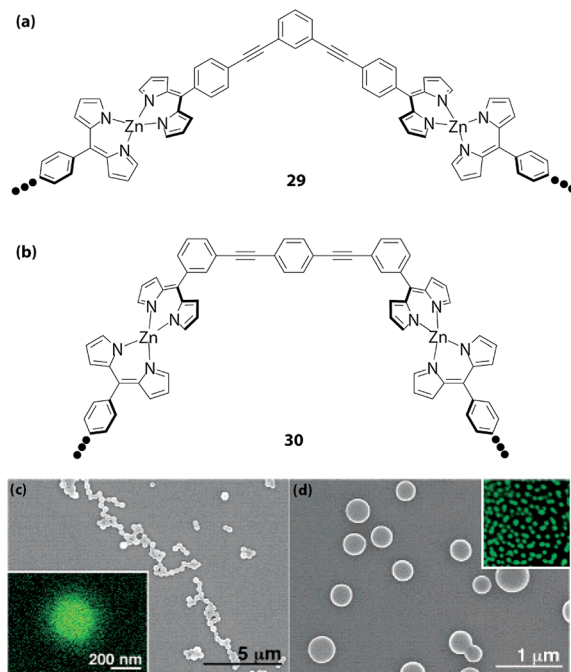
Fig. 13 One-dimensional bis(dipyrrinato)zinc(II) complex polymers (a) 29 and (b) 30 . (c) SEM image of one-dimensional coordination polymer 29 . The inset shows Zn mapping drawn by HRTEM/EDX. (d) SEM image of one-dimensional coordination polymer 30 . The inset shows a fluorescence micrograph with a 25 \mu\text{m} side of each square. Adapted with permission from ref. 73. Copyright 2006 American Chemical Society.
