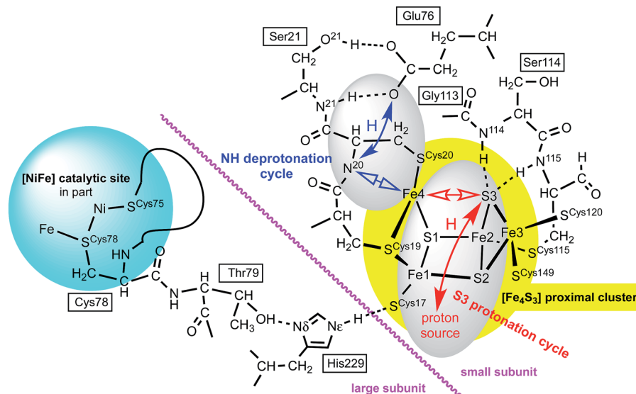
Fig. 4 Some relevant features of the model developed in this paper. Atom numbering of Re and Ec structures is used: for Hm species the link residues are Cys79, Thr80, His230. Closed arrows represent proton movements; open arrows show the movement of Fe4. The separation of the NH deprotonation cycle (blue) and S3 protonation cycle (red) is evident: details of the 'proton source' are described in the text.
