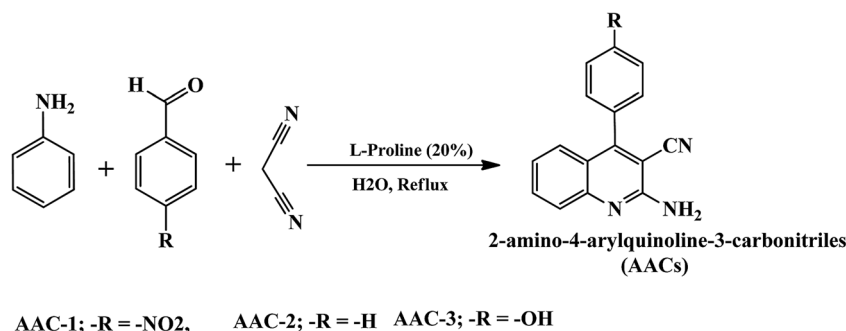
Fig. 1 Synthetic route of studied AACs.
