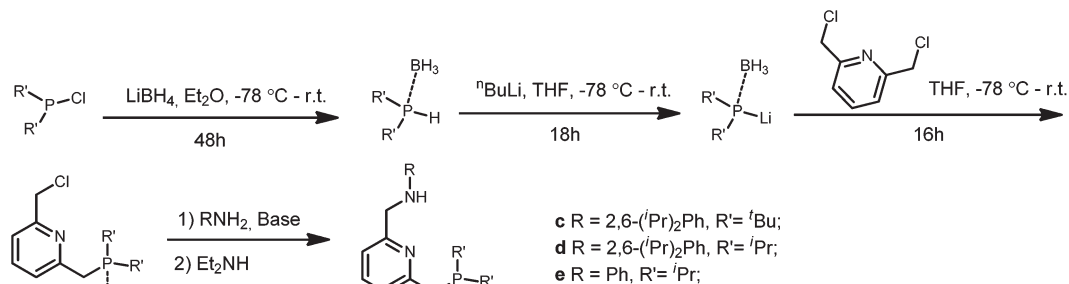
Scheme 3 Synthetic pathway [2] for the synthesis of ligands c–e .
