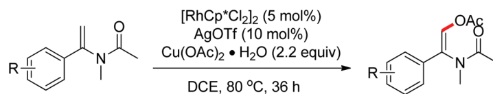
Scheme 92 Amide-assisted acetoxylation of vinyl C(sp 2 )–H bonds.
