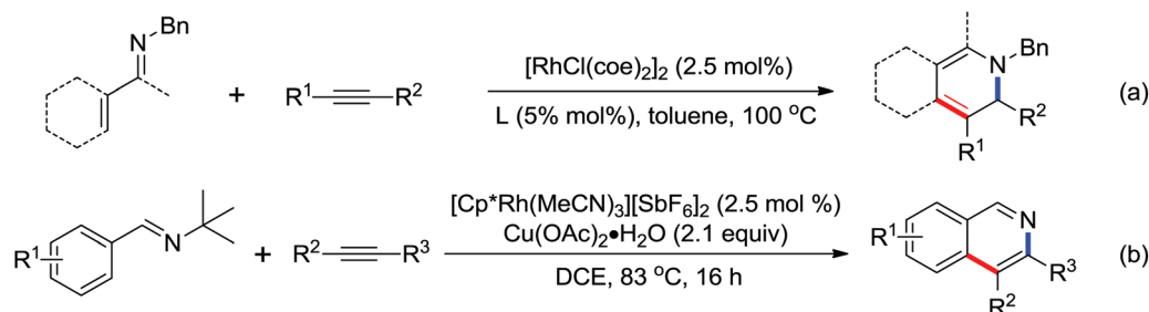
Scheme 192 Rhodium-catalyzed [4 + 2] annulation reaction.
