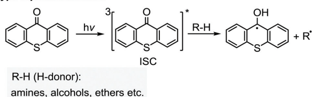
Scheme 1 Typical representation of the photolysis of the radical photoinitiators based on Type I (top) and Type II (bottom) systems with the examples of a benzoin derivative and thioxanthone, respectively.
