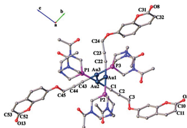
Fig. 6 Asymmetric unit of complex 1 viewed down the a -axis displaying auophilic interactions. Hydrogen atoms and solvent molecules are omitted for clarity.
