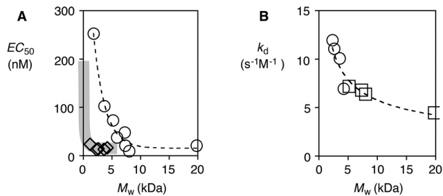
Fig. 3 (A) Dependence of EC_{50} on the molecular weight of polymers 1 (O) and 2 (◇). (B) The rate constant of depolymerization as a function of the molecular weight of polymers 1 (□) and 2 (O).
