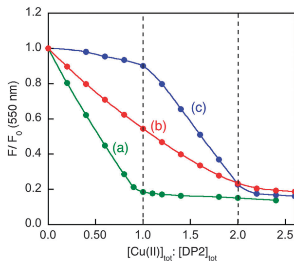
Fig. 9 Determination of Cu(II) binding stoichiometry in MOPS buffer (50 mM, pH 7.4) via titration with Cu_{aq}^{2+} of: (a) DP2 probe (2.0 μM) only; (b) a 1:1 mixture of DP2 and Aβ16 (each 2.0 μM); (c) a mixture of DP2 and peptide DAHK (each 2.0 μM).
