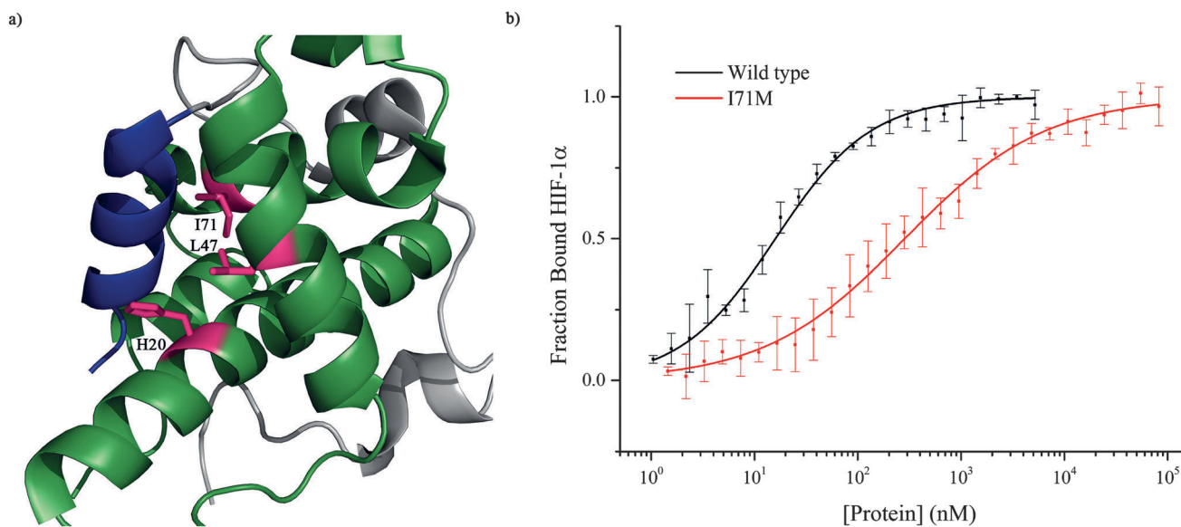
Fig. 6 Investigation of the HIF-1α helix 3 binding pocket on p300. (a) Schematic highlighting the three residues of the helix p300 binding pocket of p300 which were mutated. (b) Fluorescence anisotropy comparison of the binding of FITC-HIF-1α 786-826 to wild-type p300 (black) and mutant p300 I71M (red).
