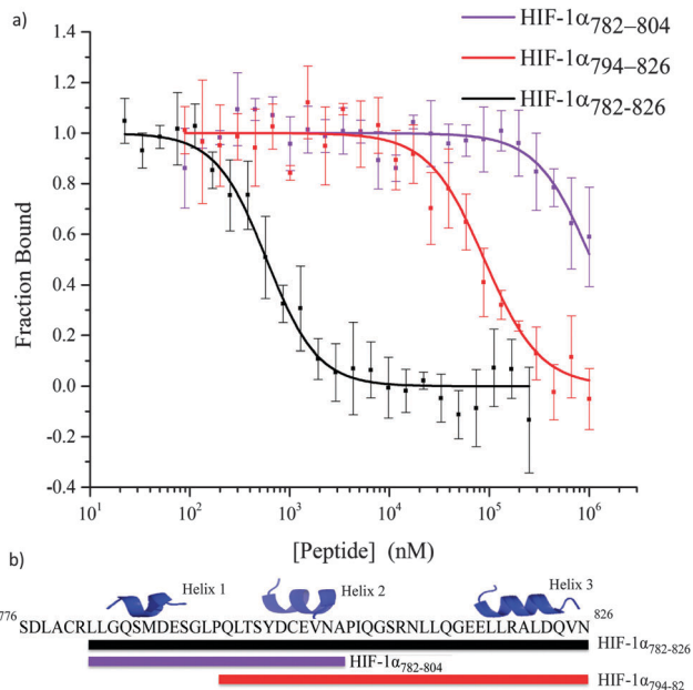
Fig. 5 Fluorescence anisotropy competition assay to test the disruption of the HIF-1α C-TAD/p300 CH1 complex by HIF-1α CTAD fragments. HIF-1α 782-826 (black) HIF-1α 794-826 (red) and HIF-1α 782-804 (violet).
