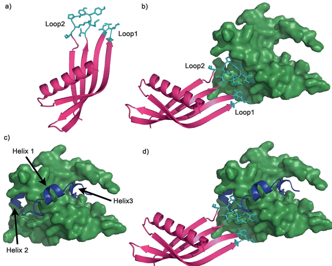
Fig. 8 Adhiron structure and potential binding model to p300. (a) Crystal structure of Adhiron, variable loops shown in cyan. (b) Adhiron Adh34 (magenta) docked to the NMR structure of p300 (green) using HADDOCK; key binding residues are shown in cyan. (c) NMR structure of HIF-1 \alpha (blue) bound to p300 (green) in the same orientation as the docked Adhiron (shown in b). (d) Overlay of the docked Adh34 (magenta) and HIF-1 \alpha (blue) bound p300 (green), highlighting Adh34 does not dock in a helix binding pocket.
