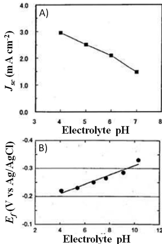
Fig. 18 (A) pH dependence of J_{sc} values ( P_{\text{in}} = 1 sun) obtained for an aqueous DSSC sensitized with N719. Electrolyte: KI 0.50 M and \text{I}_2 25 mM; (B) dependence of the Fermi level electrochemical potential ( E_f ) of the mesoporous \text{TiO}_2 electrode on the pH of the above reported electrolyte. The potential data were based on the measurement of the onset potential of dark cathodic current. Adapted and reprinted from ref. 138.
