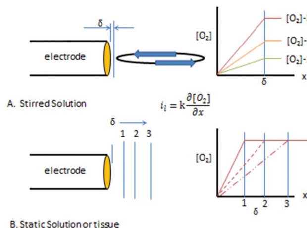
Fig. 3 (A) Concentration profiles for different [O_2] under stirred conditions. (B) Concentration profile development and diffusion layer distance ( \delta ) in a quiescent system.
