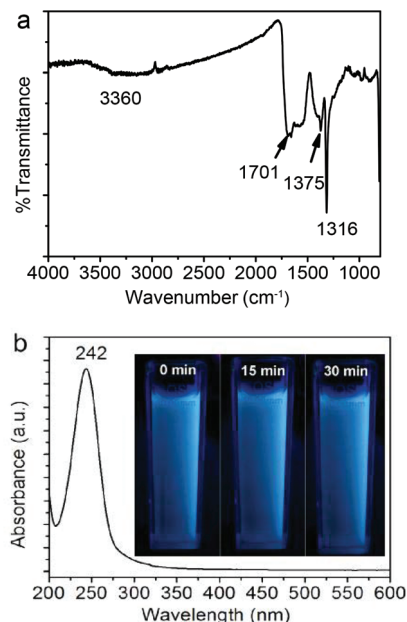
Fig. 3 (a) Typical FT-IR spectrum and (b) UV-Vis spectrum of the as-obtained \text{Fe}_3\text{O}_4\text{@C-CDs} NPs. The inset in (b) shows photographs of the aqueous dispersions of the \text{Fe}_3\text{O}_4\text{@C-CDs} NPs under UV light (365 nm) with different exposure times from 0 min to 30 min.
