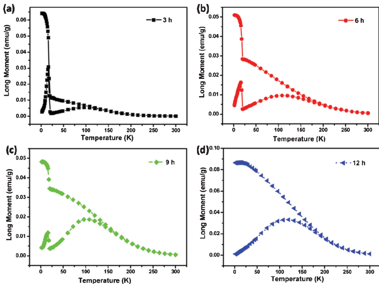
Fig. 9 (a–d) ZFC-FC curves of NiCo 2 O 4 samples at 100 Oe.
