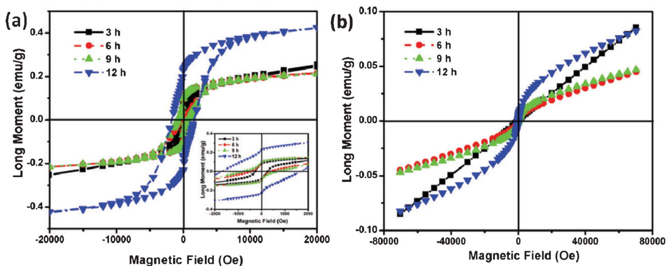
Fig. 8 (a) Low temperature 5 K hysteresis loops of NiCo 2 O 4 samples and an enlarged view at low field is shown in the inset. (b) Room temperature hysteresis loops of NiCo 2 O 4 samples.
