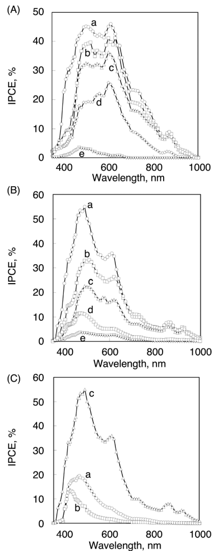
Fig. 17 (A) The photocurrent action spectra (IPCE vs. wavelength) of (a) (P(H 2 P) 16 + C 60 ) m , (b) (P(H 2 P) 8 + C 60 ) m , (c) (P(H 2 P) 4 + C 60 ) m , (d) (P(H 2 P) 2 + C 60 ) m and (e) (P(H 2 P) 1 + C 60 ) m modified OTE/SnO 2 electrodes. (B) The photocurrent action spectra of (a) (P(ZnP) 16 + C 60 ) m , (b) (P(ZnP) 8 + C 60 ) m , (c) (P(ZnP) 4 + C 60 ) m , (d) (P(ZnP) 2 + C 60 ) m and (e) (P(ZnP) 1 + C 60 ) m modified electrodes. (C) The photocurrent action spectra of (a) (P(ZnP) 16 + ImC 60 ) m , (b) (P(ZnP) 16 + PyC 60 ) m and (c) (P(ZnP) 16 + C 60 ) m modified OTE/SnO 2 electrodes. See text for the employed concentration of the individual species.
