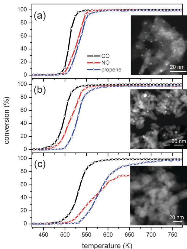
Fig. 1 Three-way catalytic activity and HAADF-STEM images of 2 wt% \text{Rh}/\text{Al}_2\text{O}_3 (a) fresh, (b) aged at 973 K and (c) aged at 1273 K.
