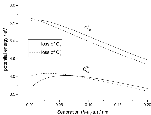
Fig. 7 Comparison between potential energy curves calculated for C_{38}^{3+} and C_{68}^{3+} undergoing either reaction step (R5) or (R6).
