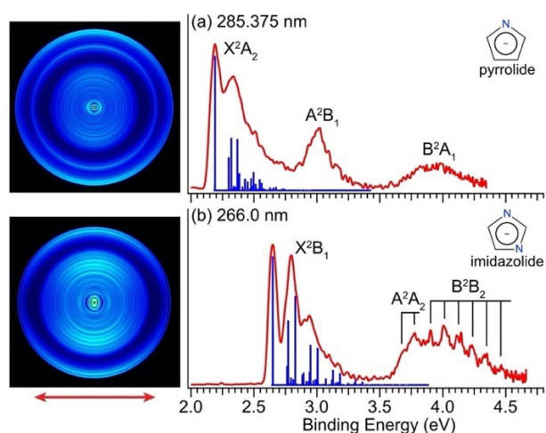
Fig. 1 PE images and spectra of (a) pyrrolide at 285.375 nm (4.3446 eV) and (b) imidazolide at 266.0 nm (4.6611 eV). The calculated FC factors for the ground electronic states are presented as blue sticks for comparison. The insets display the molecular structures of the two anions. The double arrow below the images indicates the polarization direction of the detachment laser.
