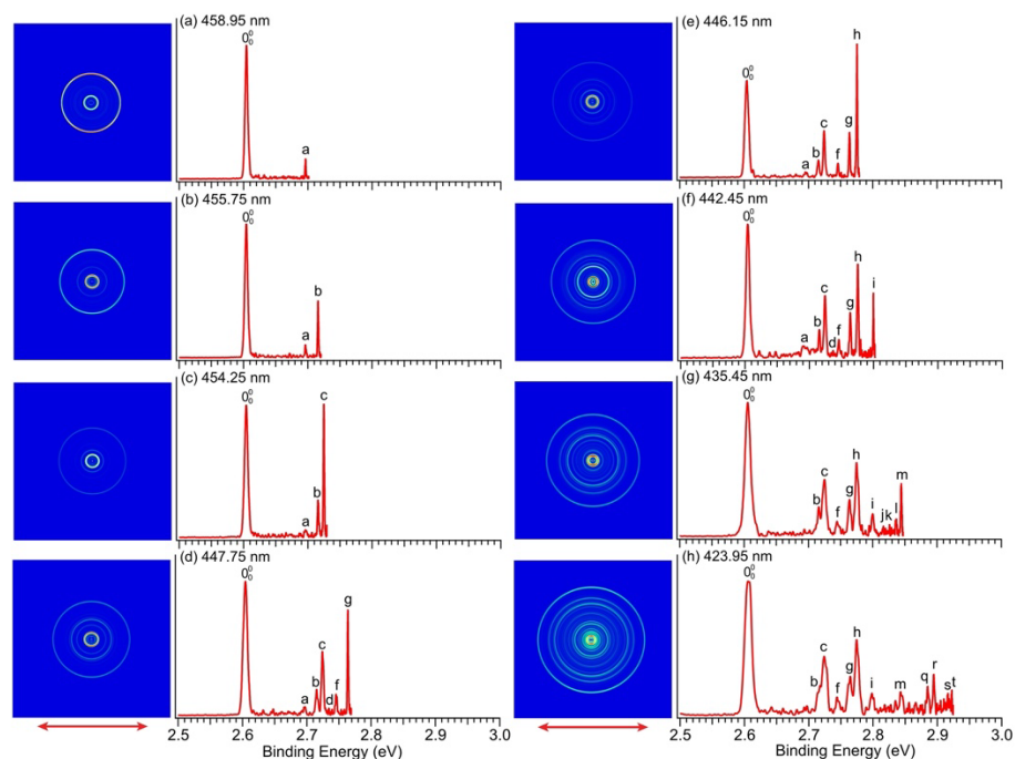
Fig. 5 PE images and spectra of the imidazolide anion at (a) 458.95 nm (2.7015 eV), (b) 455.75 nm (2.7204 eV), (c) 454.25 nm (2.7294 eV), (d) 447.75 nm (2.7691 eV), (e) 446.15 nm (2.7790 eV), (f) 442.45 nm (2.8022 eV), (g) 435.45 nm (2.8473 eV) and (h) 423.95 nm (2.9245 eV). The double arrows indicate the polarization direction of the detachment laser.
