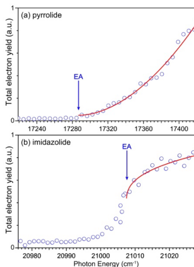
Fig. 6 Photodetachment spectra of (a) pyrrolide and (b) imidazolide. The EA of each anion is indicated by the arrow. The photodetachment spectra are fitted by the Wigner threshold law: \sigma = A * (h\nu - EA)^{l+1/2} , where A is a parameter related to the PE signal intensity, h\nu is the photon energy, and l is the angular momentum of the photoelectron. The l value is fitted to be 1.4 for (a) and -0.1 for (b).
