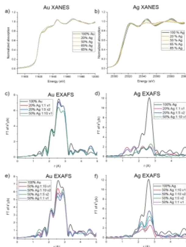
Fig. 5 Au XANES (a) shows Au 0 with altered potential at high Ag incorporation. Ag XANES (b) reveals Ag 0 character for 20 atomic % solution Ag samples, suggesting a lack of incorporation into the bulk. (c) and (d) reveal Au that shows evidence of primarily Au-Au coordination and Ag that exhibits underincorporation for the low Ag incorporation samples shown. (e) and (f) reveal differences in atomic scale coordination for samples with similar atomic % Ag, but different reductant ratios and volumes.
