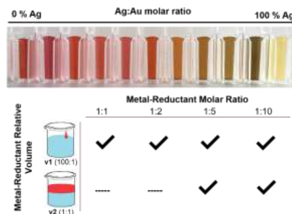
Fig. 1 Reduction parameters systematically varied in an exploration of the synthetic effects on atomic scale AgAu distributions included the Ag:Au molar ratio, which resulted in a visible change in optical absorbance wavelength (top), the metal-reductant molar ratio (bottom, right) and the volume of reductant added to the reaction (bottom, left). The volumes of reductant added consisted of either small, concentrated reductant volume (v1) or larger, diluted reductant volume (v2).
