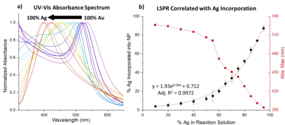
Fig. 4 a) UV-vis absorption spectra show a blue-shift in the LSPR peak position with increasing Ag incorporation. b) The shift in the LSPR position (red) tracks reciprocally with the increasing Ag atomic % incorporated into the NPs (black).
