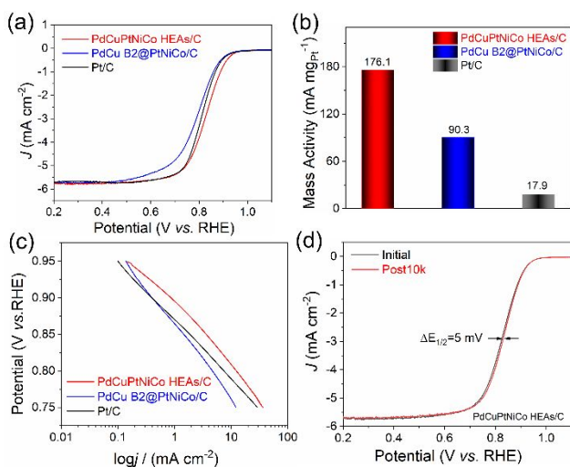
Fig. 5 (a) Evaluation of ORR performance of PdCuPtNiCo HEAs/C, PdCu B2@PtNiCo/C, and Pt/C. (a) LSV curves recorded in O 2 -saturated 0.1 M KOH solution with a rotation rate of 1600 rpm, (b) Mass activity at 0.9 V, and (c) Tafel plots. (d) ORR polarization curves of the PdCuPtNiCo HEAs/C before and after 10000 cycles.
