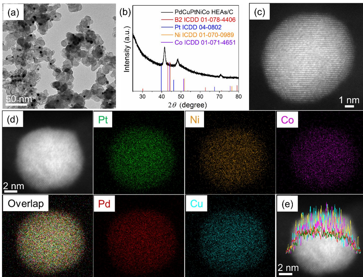
Fig. 4 Morphological and compositional characterization of PdCuPtNiCo HEAs/C: (a) TEM bright-field image, (b) XRD pattern, (c) STEM-HAADF image, (d) STEM-EDS elemental mapping images and (e) line scan profile.
