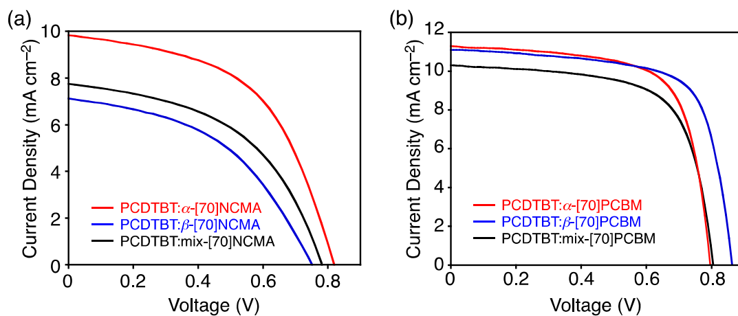
Fig. 3 Current density-voltage curves averaged from ten independent PSC devices based on (a) PCDTBT:α-[70]NCMA (red), PCDTBT:β-[70]NCMA (blue), and PCDTBT:mix-[70]NCMA (black) and (b) PCDTBT:α-[70]PCBM (red), PCDTBT:β-[70]PCBM (blue), and PCDTBT:mix-[70]PCBM (black) films.
