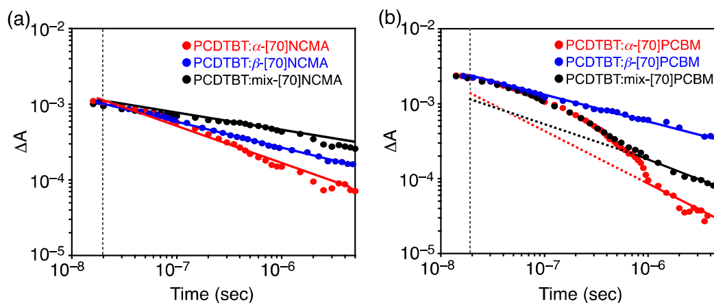
Fig. 4 Transient absorption decay kinetics of (a) PCDTBT: \alpha -[70]NCMA (red), PCDTBT: \beta -[70]NCMA (blue), and PCDTBT:mix-[70]NCMA (black) and (b) PCDTBT: \alpha -[70]PCBM (red), PCDTBT: \beta -[70]PCBM (blue), and PCDTBT:mix-[70]PCBM (black) films. Excitation and probe wavelengths are 532 nm and 970 – 1000 nm. The \Delta A signal intensities are normalized at 20 ns. Fitting lines with power-law decays (straight lines on the log-log plot) are also shown. Dotted lines for PCDTBT: \alpha -[70]PCBM and PCDTBT:mix-[70]PCBM in (b) are extrapolated from the power-law decays. The vertical gray dotted lines are located at 20 ns.
