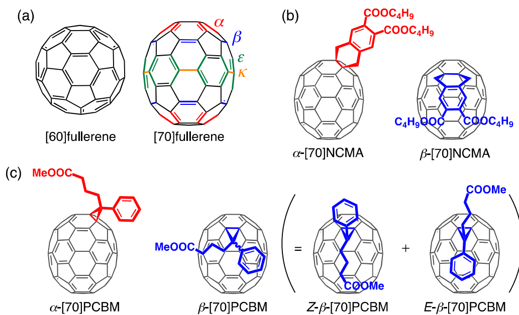
Fig. 1 (a) Structures of [60]fullerene and [70]fullerene. \alpha -, \beta -, \varepsilon -, and \kappa -type [6,6]-bonds of [70]fullerene are represented by red, blue, green and orange lines. (b) Structures of [70]NCMA isomers. (c) Structures of [70]PCBM isomers.
