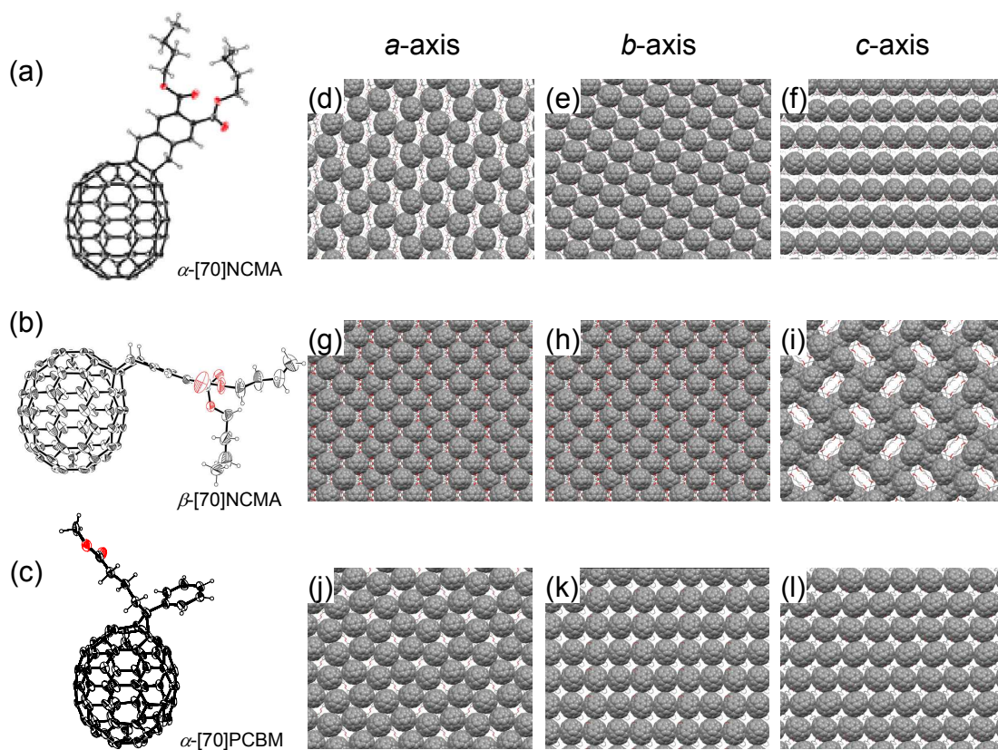
Fig. 2 X-ray crystal structures of (a) \alpha -[70]NCMA, (b) \beta -[70]NCMA, and (c) \alpha -[70]PCBM. Thermal ellipsoids represent 30% probability. Minor disorder components and solvent molecules are omitted for clarity. X-ray crystal packing structures of (d-f) \alpha -[70]NCMA, (g-i) \beta -[70]NCMA, and (j-l) \alpha -[70]PCBM with solvent molecules along with (d,g,j) a -axis, (e,h,k) b -axis, and (f,i,l) c -axis.
