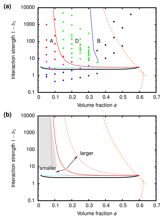
Fig. 7 (a) The predicted gravitationally-shifted A-D boundary, Eq. 7, overlaid onto our data. (b) The scaling of the transition between A and D with particle size. The grey area marks regime A from previous work 25 on colloidal gels with smaller particles.
