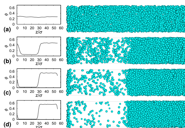
Fig. 3 Simulated equilibrium gas-liquid coexistence in an elongated box using EDMD. Well width = 0.1D . Well depths \epsilon/k_B T = (a) 2.0, (b) 2.2, (c) 2.3 and (d) 2.4, corresponding to 1 - b_2 = 2.11, 2.66, 2.97 and 3.32 respectively. We show snap shots of the simulation box (right) and the corresponding volume fraction profiles along the box (left)
