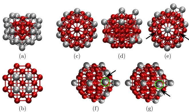
Fig. 3 Ball-and-stick representation of biminima for \text{Cu}_{13}\text{Ag}_{25} (a), \text{Cu}_{34}\text{Ag}_4 (b) and \text{Cu}_{44}\text{Ag}_{11} (c-g). Cu atoms are smaller and coloured red, Ag atoms are larger and coloured grey. Arrows in (e) indicate the vertex sites from which two Ag atoms have been dislodged. The subtle geometric differences between (f) and (g) are highlighted by a circle around a most shifted Ag atom and an arrow pointing to a destroyed/created nearest-neighbour “bond”.
