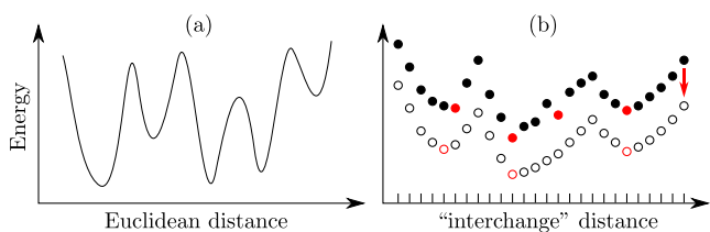
Fig. 1 A schematic diagram illustrating how the energy of a nanoalloy might vary along a continuous reaction coordinate (a) or a sequence of atom swaps/interchanges (b). In (b), the filled symbols correspond to a swap sequence at fixed geometry, whereas the open symbols illustrate the effect of quenching.
