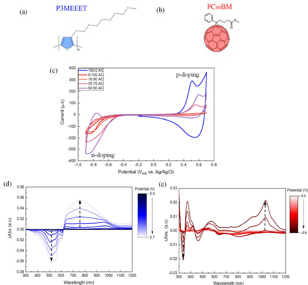
Fig. 1 Chemical structures of (a) P3MEEET and (b) PC 60 BM. (c) Cyclic voltammetry of P3MEEET:PC 60 BM as-cast blends in 0.1 M KCl. The voltammogram corresponds to the 10th scan. (d) and (e) Spectroelectrochemical absorption changes of as-cast 50 : 50 w : w% blend, measured at +0.7 V to -0.9 with voltage steps of 0.1 V. Blue curves represent the measured absorption changes in positive bias and hence show changes in the polymer doping, while red curves are measured in negative bias and show doping of the fullerene.
