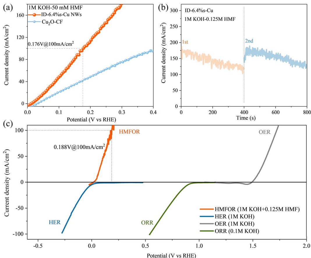
Fig. 6 (a) LSV curves and of ID-6.4%Cu NWs and Cu 2 O-CF. (b) Stability test of ID-6.4%Cu in 1 M KOH and 0.125 M HMF. (c) LSV curves of ORR in 0.1 M KOH by Fe single atom for Zn-air battery, HER in 1 M KOH by Pt foil, OER in 1 M KOH and HMFOR in 1 M KOH with 0.125 M HMF by ID-6.5%Cu.
