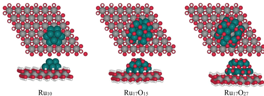
Fig. 8 Optimized structures of Ru 10 , Ru 17 O 15 and Ru 17 O 27 clusters over a Ni(OH 2 ) (100) layer.
