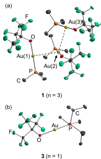
Fig. 2 X-ray crystal structures of (a) trimeric [\{\text{Au}(\text{OC}(\text{CF}_3)_3)\{\text{PMe}_3\}_3] (1) and (b) monomeric [\text{Au}(\text{OC}(\text{CF}_3)_3)\{\text{P}^i\text{Pr}_3\}] (3). In compound 1, the \text{CF}_3 groups of the \text{OC}(\text{CF}_3)_3 ligands on Au(2) and Au(3) are disordered over two positions, and only the major disorder component (83.3(5)% for the ligand on Au(2), and 61.0(8)% for the ligand on Au(3)) is shown. Hydrogen atoms are omitted for clarity and thermal ellipsoids are at 50% probability.
