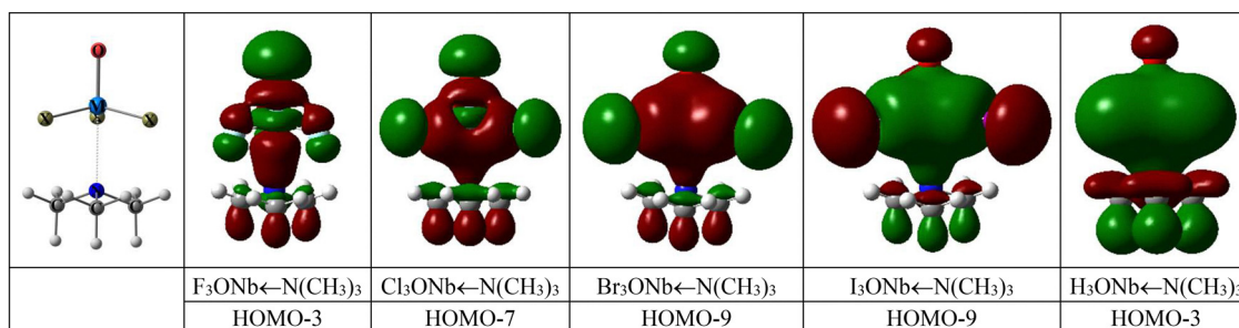
Fig. 2 Representations of \text{X}_3\text{ONb} \leftarrow \text{N}(\text{CH}_3)_3 molecular orbitals that are bonding between the \text{NbOX}_3 and \text{N}(\text{CH}_3)_3 fragments. The position of each orbital relative to the highest occupied molecular orbital (HOMO) for the complex is indicated. All of the MO pictures share the same orientation. That common orientation is depicted on the left.
