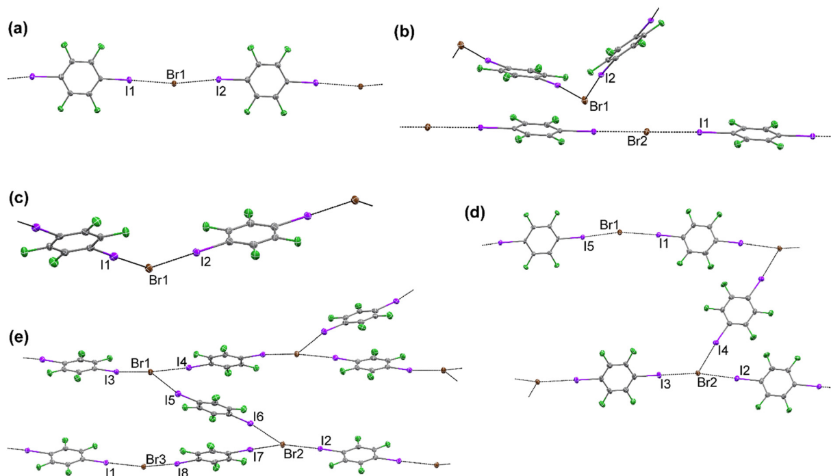
Fig. 2 Halogen bonding in NMe 3 BzBr:p-F 4 DIB (a), 2(NMe 3 BzBr):2(p-F 4 DIB):MeCN (b), NMe 3 BzBr:p-F 4 DIB:Acetone (c), 4(NMe 3 BzBr):5(p-F 4 DIB) (d), and 3(NMe 3 BzBr):4(p-F 4 DIB) (e). Solvent molecules and hydrogen atoms are omitted for clarity. Atomic displacement ellipsoids are displayed at the 50% probability level.
