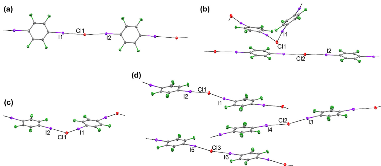
Fig. 1 Halogen bonding in NMe 3 BzCl:p-F 4 DIB (a) (viewed down the c axis), 2(NMe 3 BzCl):2(p-F 4 DIB):MeCN (b) (viewed down the c* axis), NMe 3 BzCl:p-F 4 DIB:Acetone (c) (viewed down the b axis), and 3(NMe 3 BzCl):3(p-F 4 DIB):2(CHCl 3 ) (d). Solvent molecules and hydrogen atoms are omitted for clarity. Atomic displacement ellipsoids are displayed at the 50% probability level. Carbon atoms are gray, fluorine atoms green, iodine atoms purple, chlorine atoms red, and bromine atoms brown.
