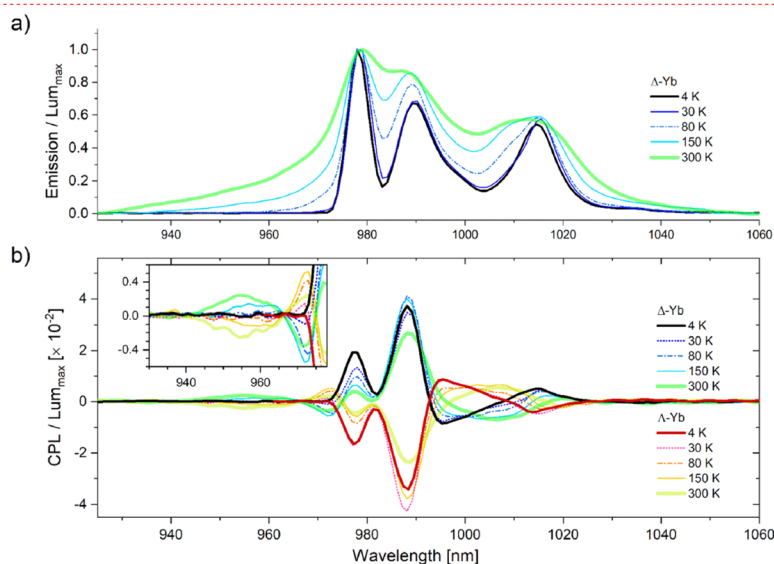
Scheme 43 (Above) Chemical structures of the ligands and Ln complexes [\text{Yb}(\text{S,S/R,R-L}^{\text{NHHex}_2})_3(\text{OTf})_3] , adapted from ref. 103. (Below) Variable temperature spectra of the two \text{Yb}^{3+} complexes in PDMS at 4, 30, 80, 150 and 300 K. (a) Variable temperature-luminescence spectra for D-Yb. (b) Variable temperature-CPL spectra. Inset shows the enlarged region of hot bands. Reproduced from ref. 103 with permission from the Royal Society of Chemistry, copyright [2024]. 103
