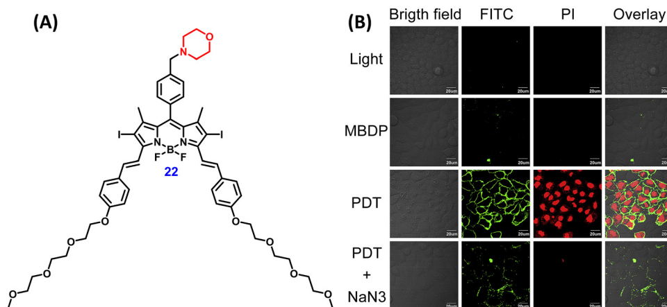
Fig. 27 (A) Chemical structure of probe 22 . (Redrawn the ChemDraw structures from ref. 100) (B) confocal fluorescence images of MCF-7 cells treated with probe 22 under various conditions: light irradiation, probe alone, and pre-treatment with ^1\text{O}_2 scavenger \text{NaN}_3 demonstrating its PDT efficacy. Reproduced with permission from ref. 100, Copyright 2017 Elsevier.
