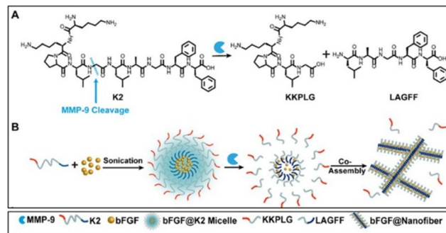
Fig. 7 Schematic illustration of bFGF@Nanofiber formation. (A) Chemical structure of the MMP-9-responsive peptide K2. (B) Transformation of bFGF@K2 micelle to bFGF@Nanofiber upon MMP-9 cleavage. Reproduced from ref. 53.
