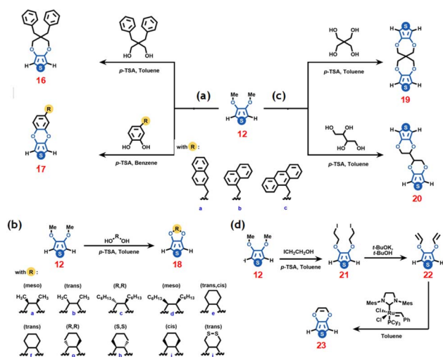
Scheme 4 O-alkylation based on a transesterification reaction for the synthesis of (a) dibenzyl propyleneedioxythiophene and 3,4-phenyleneedioxythiophene derivatives, (b) chiral EDOT derivatives, (c) bis-alkoxythiophenes and (d) 3,4-vinyleneedioxythiophene (VDOT).
